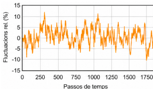
Figura 1.10: Fluctuacions relatives per N = 500 .
